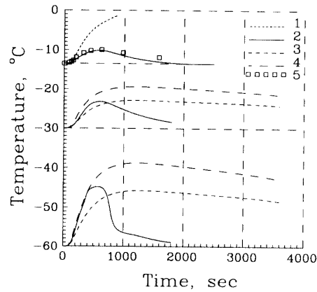
Fig. 7. Temperature at center of the ice core affected by borehole fluids: 1–water, 2–EWS, 3–kerosene ( h_s=5 mm), 4–kerosene ( h_s=30 mm), 5–experimental data.
