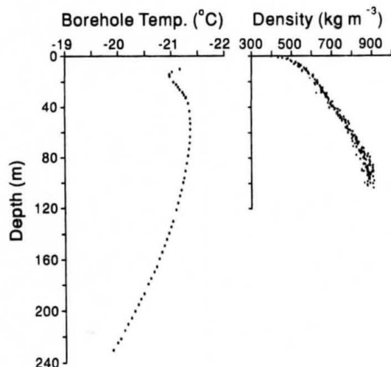
Fig. 2. The temperature profile was measured in the 1989-90 Dyer Plateau borehole and densities were measured to 100 m along core 1.
